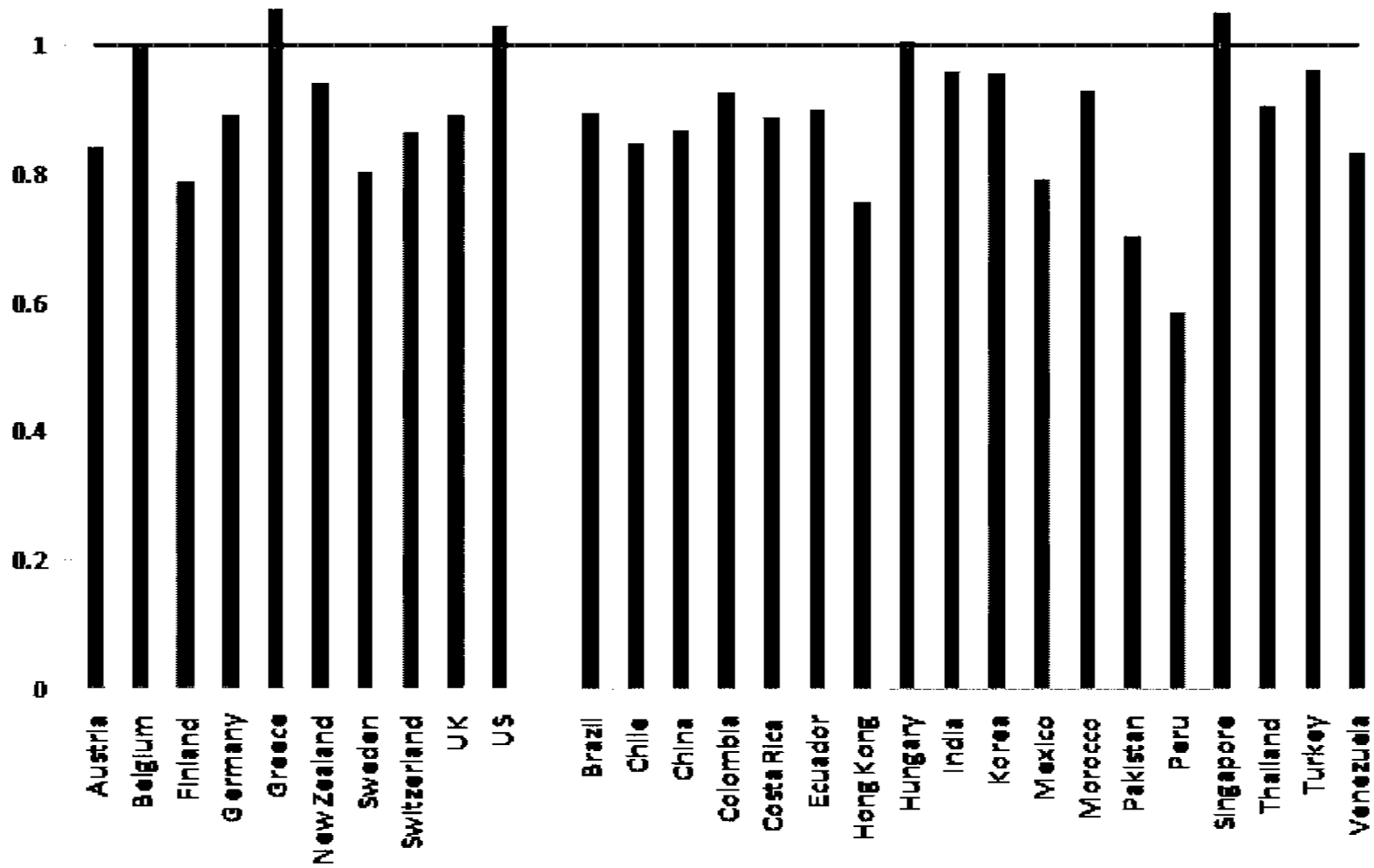
Figure 3. The Estimated AR(1) Coefficients
