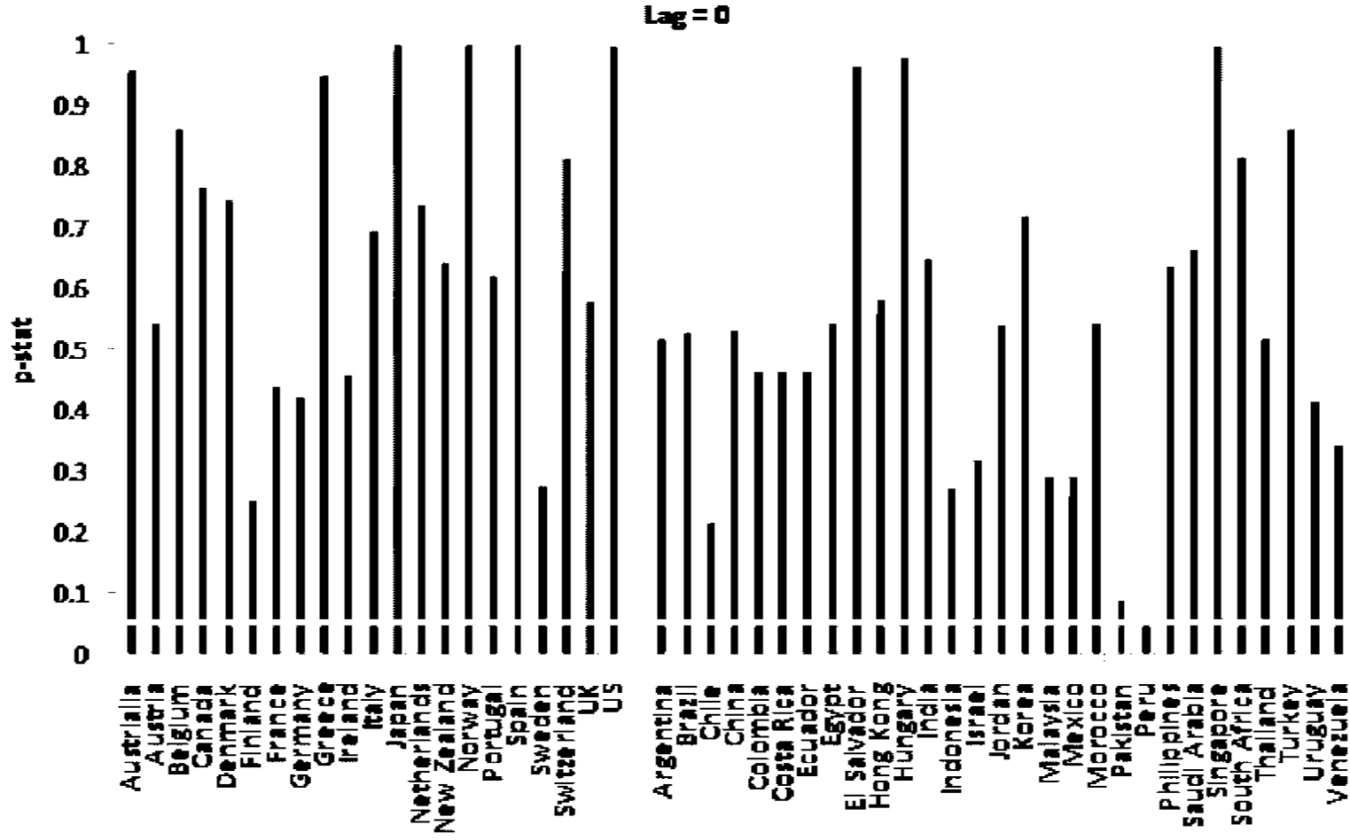
Figure 2. The Order of Integration of Net Foreign Assets Positions
